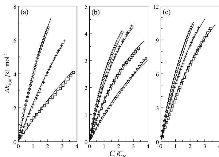
Fig. 2 Calorimetric titrations for the complexation of Eu(III) by malonamides in 10% DMSO/AN. (a) Eu/THMA: C_M^0 = 32.4 (○), 16.2 (+), 8.58 \text{ mmol dm}^{-3} (□); (b) Eu/MeTHMA: C_M^0 = 33.85 (○), 25.39 (+), 16.92 (□), 8.46 \text{ mmol dm}^{-3} (▽); (c) Eu/DMDBMA: C_M^0 = 33.35 (○), 25.01 (+), 16.68 \text{ mmol dm}^{-3} (□). The lines are calculated by using the formation constants and enthalpy values in Table 1.
